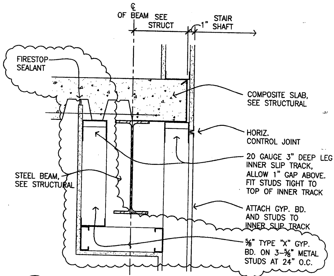
5 1-HR PARTITION AT STAIR SLAB SIM • RATED PARTITION AND PARALLEL BEAM 1 1/2" = 1'-0"
